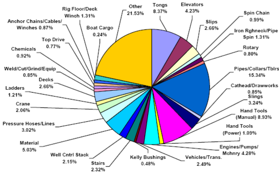
Total Industry Recordable Incidents by Equipment (Chart 10) Based on 4134 Incidents
